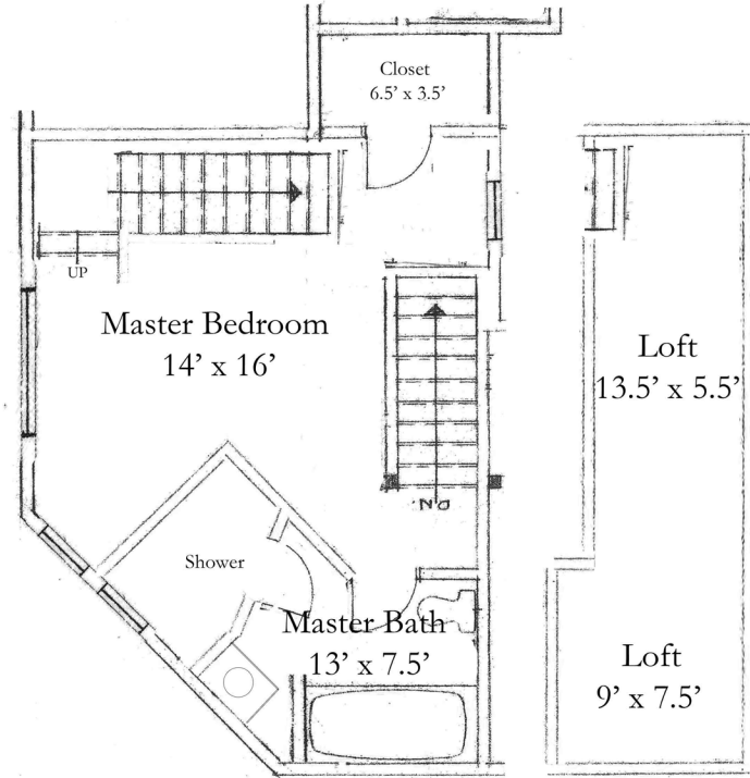
Upper Level II
